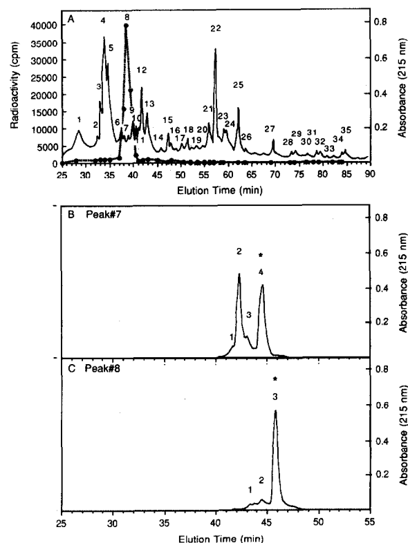
Fig. 1. HPLC profile of tryptic peptides derived from \text{p44}^{\text{mpk}} -phosphorylated MBP. (A) The peptides were resolved on a C-4 reverse phase column (unbroken line) and the corresponding radioactivity in each fraction was quantitated by liquid scintillation counting (*). The recovery of radio-label in the major peptide peaks was 38\% . (B) Peak no. 7 from panel A was rechromatographed on a C-18 reverse phase column. The radioactivity in peak nos 1, 2, 3 and 4 was 145, 345, 225 and 4650, respectively. The recovery of radio-label in peak no. 4 was 38\% . (C) Peak no. 8 from panel A was rechromatographed on a C-18 reverse phase column. The radioactivity in peak nos 1, 2 and 3, was 615, 1235, and 9935, respectively. The recovery of radiolabel in peak no. 3 was 28\% . The peptide peaks were monitored at wavelengths 215 and 280\ \text{nm} , but only the data from 215\ \text{nm} is shown (unbroken line).
